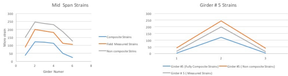
Fig. 18. Comparison of measured strains and computed for non-composite and composite cross-section
