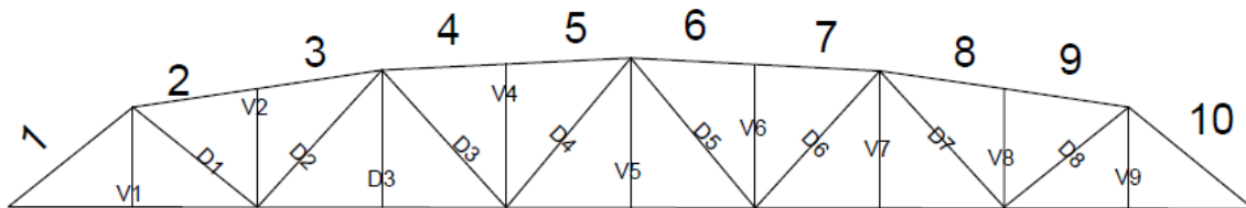
Fig. 29. Plan of the truss
