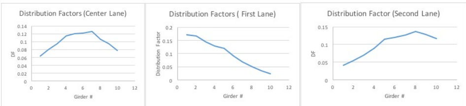
Fig. 17. Girder Distribution Factors based on measured strains in the midspan depending on the transverse position of load
